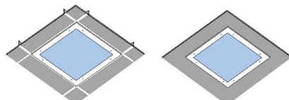
Overlapping Door in T-bar Grid Ceiling Overlapping Door Flanged
